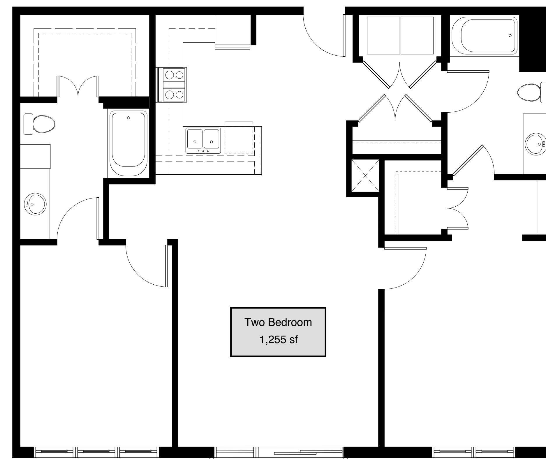
3 TWO BEDROOM UNIT A-101 SCALE: 1/4" = 1'-0"
